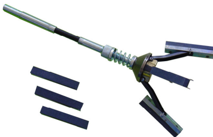
KA-4280 Brake Cylinder Hone
