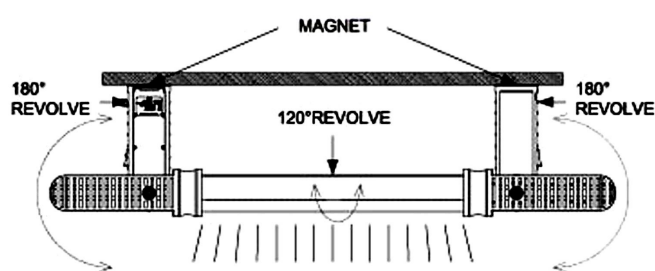
Attaching on metal surface from top or under
