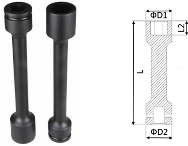
Material: SCM440
