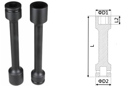
Material: SCM440
