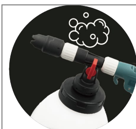
Attaching the foam jet nozzle and opening the valve to use as Foam Gun
