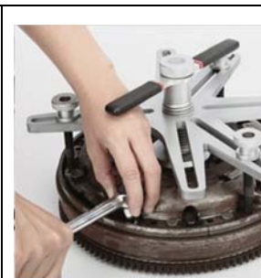
The face spanner is a releasing tool for the SAC clutches with locking element used on VW/Audi/Skoda/Seat.
